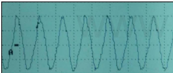
3.8 MHz carrier frequency before ray tube.
