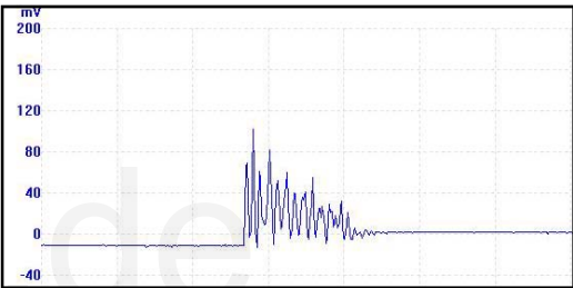
Spark gap damped waveform
